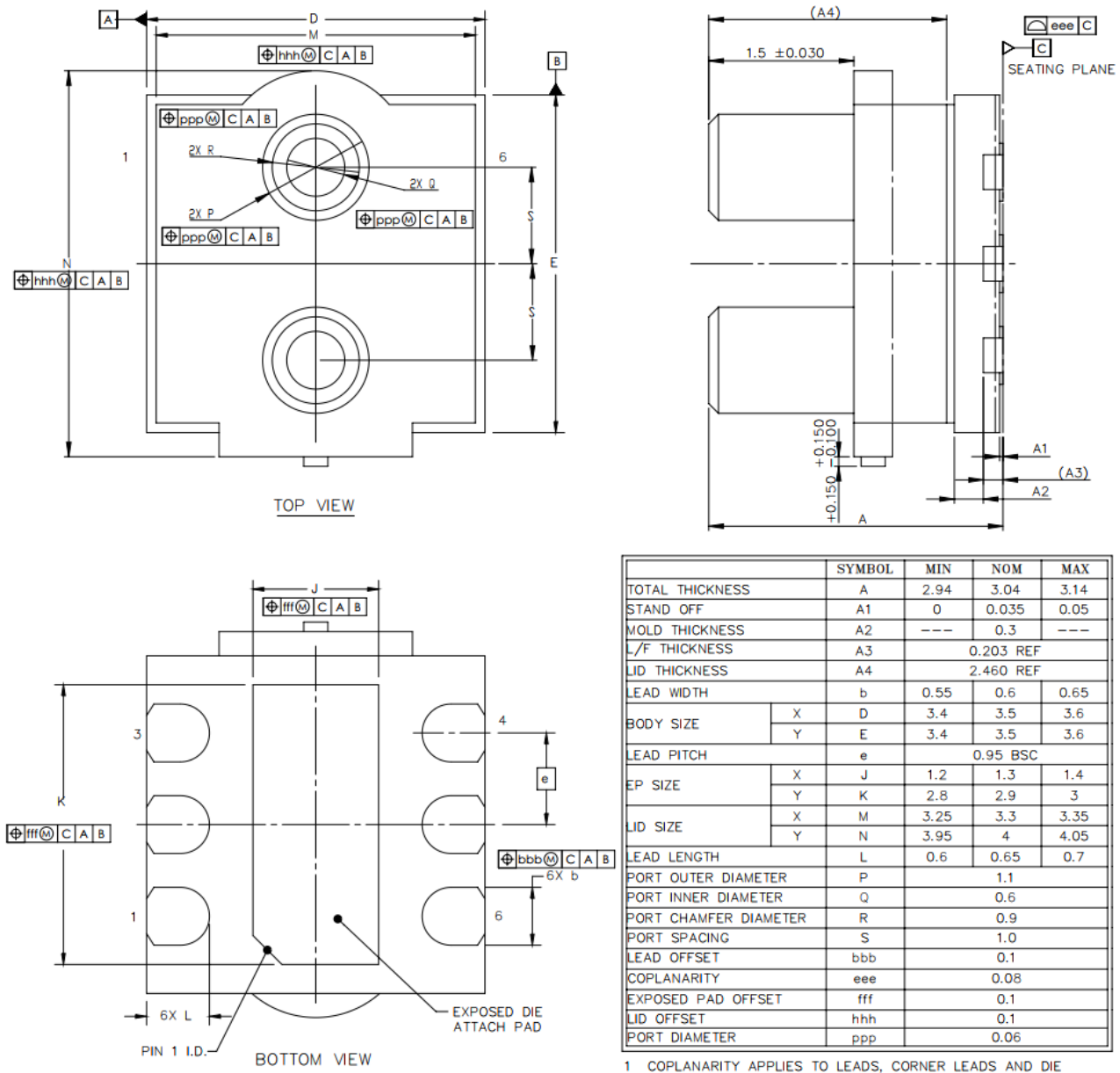
Figure 9: Package dimensions
