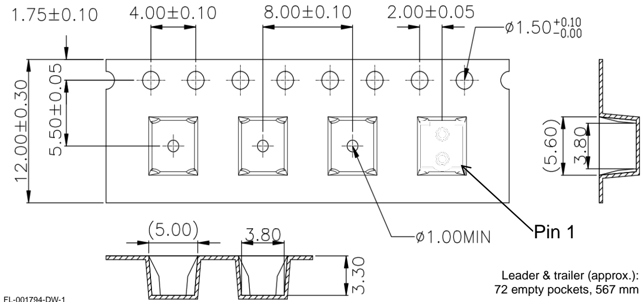
Figure 11: FLS-110-TR07 Tape Dimensions
